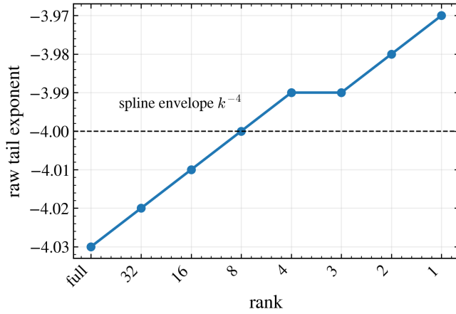
Figure 4: The 1D CPWL exponent remains pinned near -4 . This negative result is theoretically expected and motivates measuring learned Fourier recovery instead.
