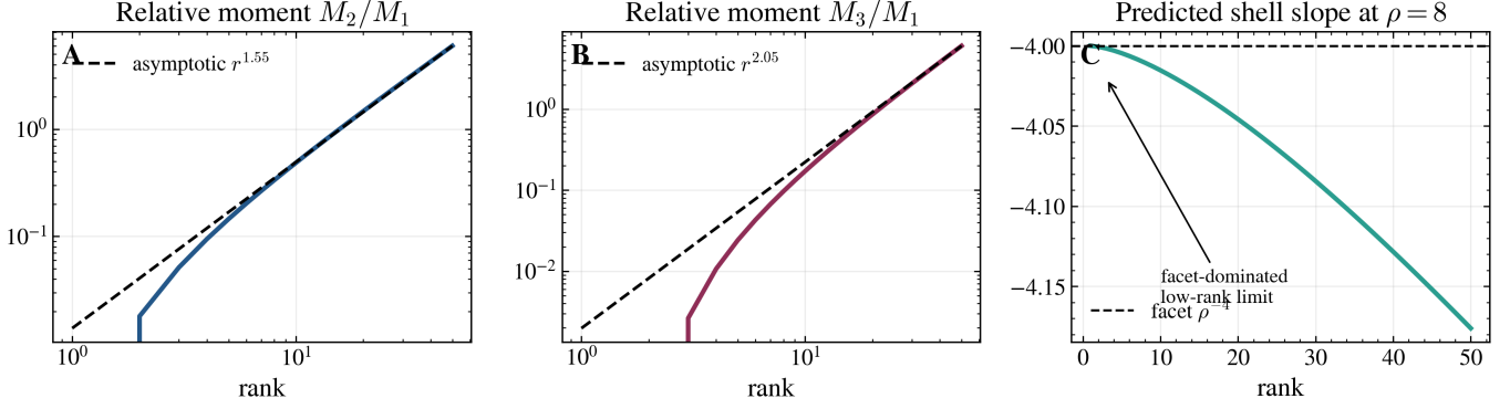
Figure 2: Combinatorial face-moment proxy. Increasing rank increases the relative mass of high-codimension intersections; low rank keeps the finite-shell slope closer to the facet-dominated CPWL exponent. This is the theory-side phase transition predicted by (22).
